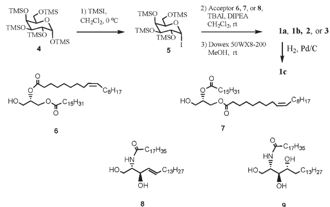
Scheme 1 Synthesis of target compounds.
