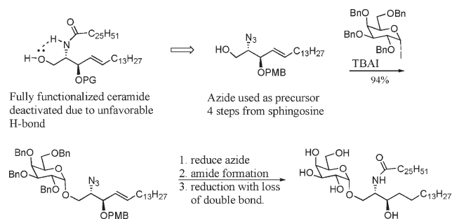
Fig. 2 First generation synthesis requires multiple protection–deprotection steps.
