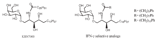
Fig. 1 Analogs of naturally occurring \alpha -GalCer from Agelas mauritianus .
