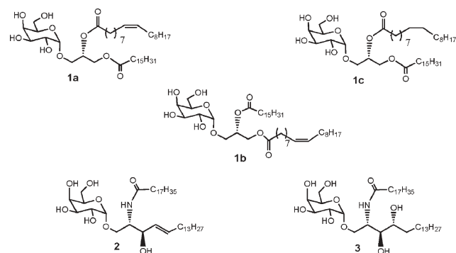
Fig. 3 Targeted bioactive glycolipids.
